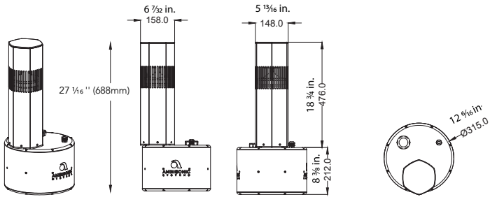
Orthographic View
